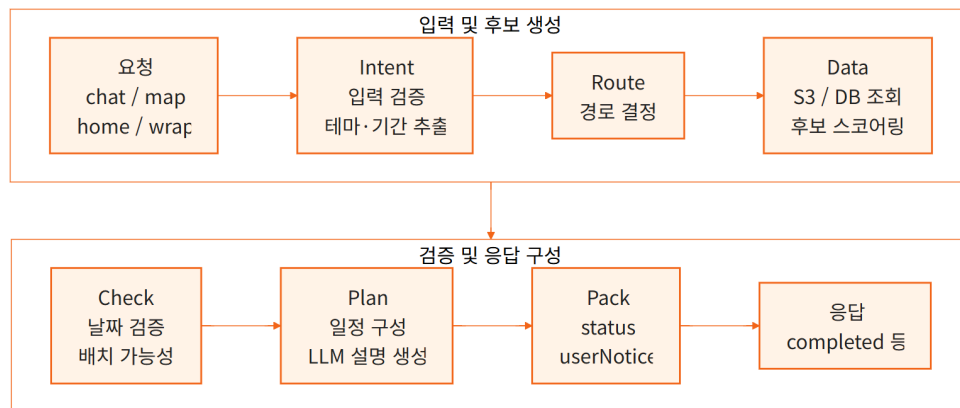
LangGraph 실행 Pipeline
