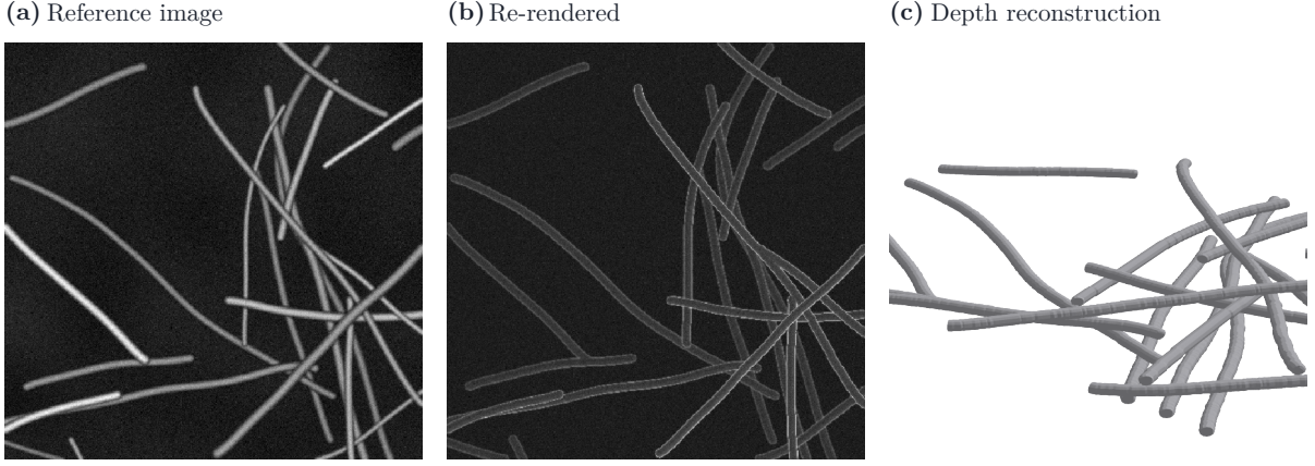
Figure 9. Depth reconstruction of a synthetic scene from its binary axis mask. The panels show the rendered greyscale image, a forward-model re-rendering from the reconstructed depths and radii, and the inferred strand stack. The re-rendering is a visual consistency check, not a scored quantity. The scene is 512 px across in the generator’s pixel units.
