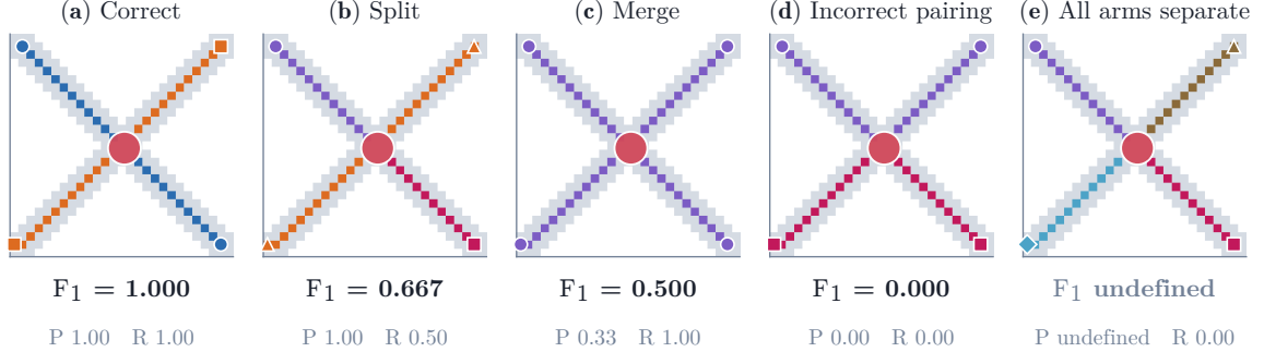
Figure 6. Illustration of the endpoint metric on the smallest case that contains a crossing. The scorer removes a neighbourhood of the junction (red) and evaluates, for each of the six pairs of the four remaining arms, whether the grouping joins it as the reference (a) does; arms sharing a tip marker belong to the same instance. Splits (b) reduce recall and merges (c) reduce precision; the all-separate grouping (e) produces no pair, so precision and F_1 are undefined rather than zero, one reason the adjusted Rand index and variation of information are reported alongside.
