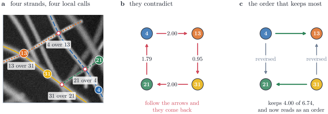
Figure 5. Why the order is solved for a whole component rather than one crossing at a time, on a contradiction the stage met on a development scene. (a) Four strands and the four calls the local evidence made at their crossings. (b) Those calls as a graph: each arrow points from the strand called upper to the one called lower, and following them returns to where it started, so no stack of heights satisfies all four. (c) The order that satisfies the most evidence by weight keeps the two heaviest calls and reverses the two lightest, including the weakest at 0.95. The reversals are recorded, not discarded. Layer numbers are not shown: a strand’s layer follows from its whole component, and these four sit in a scene of seven.
