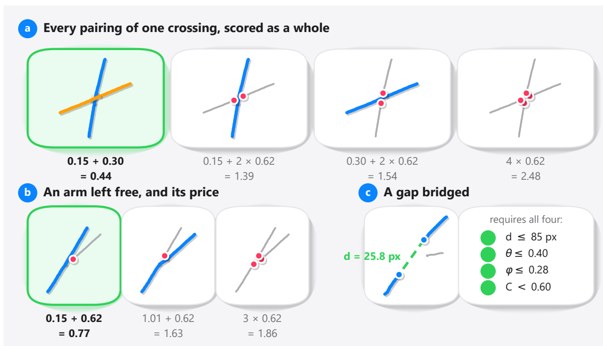
Figure 3. Every decision the linker makes, on the nodes it made them at. Every number is measured and every arm is the skeleton it was measured from, smoothed only enough to lift the raster staircase and rotated rigidly, so every angle shown is the one the cost was computed on. (a) Every pairing the admissibility gate allows at a four-arm crossing on a development scene, each scored as a whole: its edge costs plus the price p_i = 0.62 of each arm it leaves free, marked. The green card is the one returned. Two further pairs, at 3.15 and 3.33, exceed p_i + p_j = 1.24 and are never offered. (b) A three-arm node on another development scene, where an admissible edge is declined on the total rather than on its own cost. (c) A gap link, which must clear all four gates at once.
