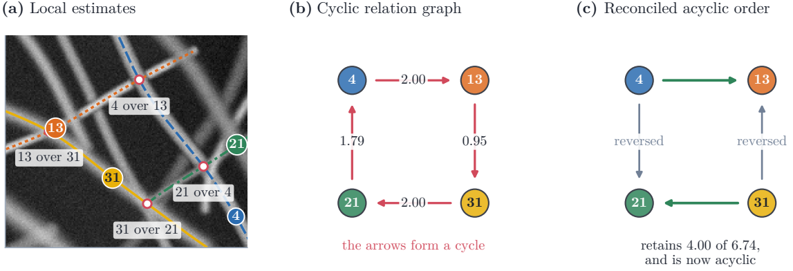
Figure 6. Resolving contradictory local depth estimates. (a) Four strands and their estimated crossing orders. (b) The corresponding graph, with arrows from the estimated upper strand to the lower strand. The directed cycle prevents a consistent height assignment. (c) The selected order retains the two highest-weight estimates and reverses the two lowest-weight estimates. Reversals are recorded with their original scores. The four strands shown belong to a seven-strand scene; layer assignments depend on the complete connected component.
