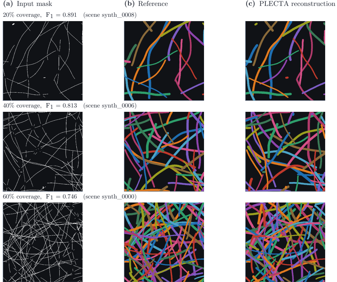
Figure 8. Segmentation at three coverage levels, each the scene closest to the median F_1 of its stratum, shown as a horizontal window of the scene. Columns: the degraded input mask, the overlap-aware reference, and PLECTA’s strands at their fitted widths. The score beside each row is the grouping’s, not the rendering’s. Strand colours are arbitrary and not matched between columns.
