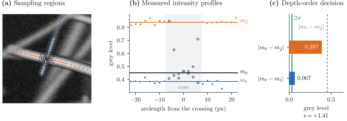
Figure 5. Local depth evidence at a crossing angle of 83.8^\circ , selected for clarity. Positions and intensities are taken from the stage output. (a) Core samples (open dots) and flank samples (filled dots), with flanks kept clear of the other strand. (b) Intensity along each strand: the pooled core median m_c is closer to strand i 's flank median than to strand j 's, supporting i as the upper strand. (c) Intensity mismatches used to calculate s , normalised by the larger of the flank-median separation and twice the local noise estimate (Supplementary Section S2).
