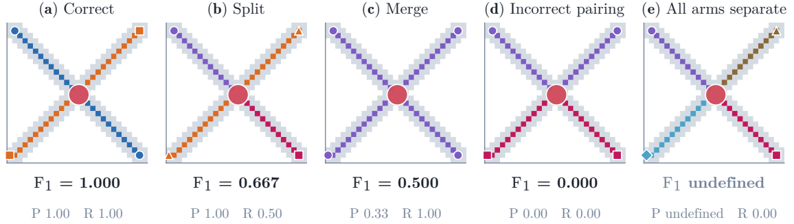
Figure 7. Pairwise scoring at a crossing. Removing junction pixels (red) leaves four arms and six fragment pairs. Tip markers identify arms assigned to the same strand. (a) Reference grouping. (b) A split reduces recall. (c) A merge reduces precision. (d) Incorrect pairing changes strand identities. (e) Separating every arm produces no predicted positive pair, so precision and F 1 are undefined.
