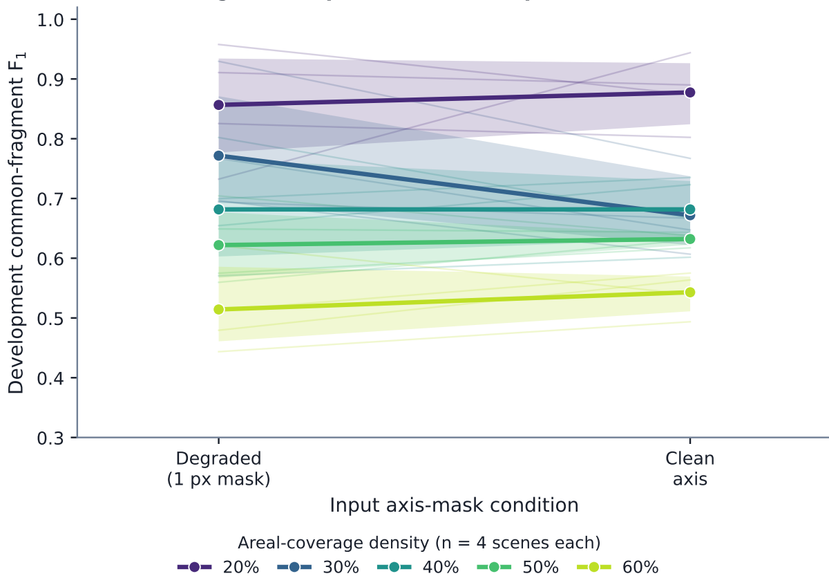
Clean vs. degraded input mask (development scenes)
