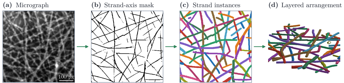
Figure 1. From micrograph to individual strands. (a) A fixed central crop of a carbon-nanotube SEM field. (b) The strand-axis mask from the upstream segmenter. (c) PLECTA segmentation output. (d) The layered arrangement estimated for the same instances.
