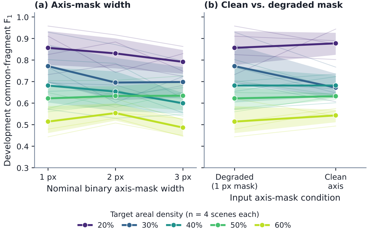
Figure 7. Sensitivity of the common-fragment F_1 to the input representation, by target areal density (Section 3.2); panels as labelled. Curves are means over 4 scenes per level (20 total); bands are 95% bootstrap CIs preserving within-scene pairing (10 000 replicates).
