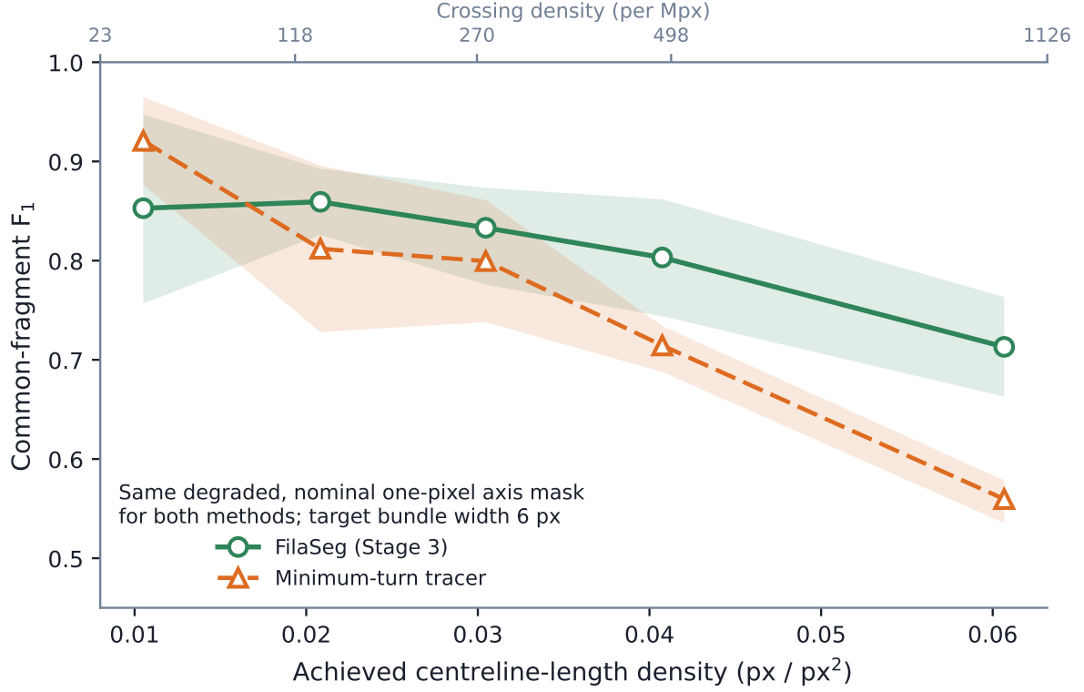
Figure 8. Centreline-length density sweep (Section 3.2): common-fragment F_1 for FilaSeg Stage 3 and the minimum-turn tracer against achieved centreline-length density, paired scene by scene at the single inert target bundle width of 6 px. Bands are 95% bootstrap CIs of the mean ( n = 4 seeds per centreline-length density level, 10 000 replicates).
