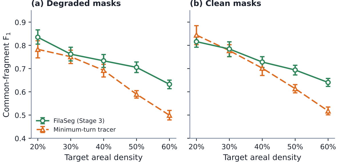
Figure 4. Common-fragment F_1 for FilaSeg Stage 3 and the minimum-turn tracer, by target areal-density level: (a) predefined degraded mask; (b) secondary, non-predefined analysis on the same 125 scenes with the undegraded one-pixel mask. Per-density means; 95% bootstrap CIs (25 scenes/level).
