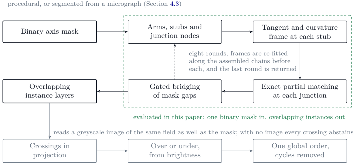
Figure 1. Where PLECTA sits. A single binary axis mask is the method’s only input, and every result in this paper measures the stage inside the dashed boundary: one binary mask in, overlapping instance layers out. The two matchings are re-made over eight rounds as frames sharpen along the assembled chains, and the last round is returned. The depth stage reads a greyscale image of the same field in addition to the mask, adds a third dimension without revising any identity, and abstains at every crossing when no image is supplied.
