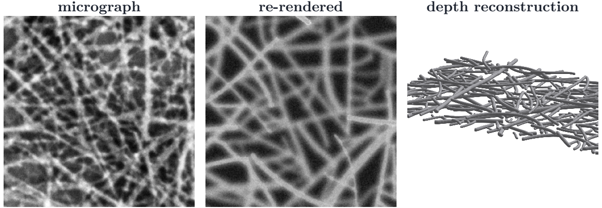
Figure 10. The same comparison on a real CNT SEM field, reconstructed from the manual annotation’s axis. Nothing here is scored. No depth ground truth exists for real SEM – the annotation records which pixels belong to which filament, not which filament passes in front – so this shows the stage runs end to end on real data and re-renders to something recognisable, not that the depths are right. The forward model’s appearance parameters are fitted to this micrograph, so the residual quoted beneath the panel is in-sample and is a sanity check rather than a measure of reconstruction quality.
