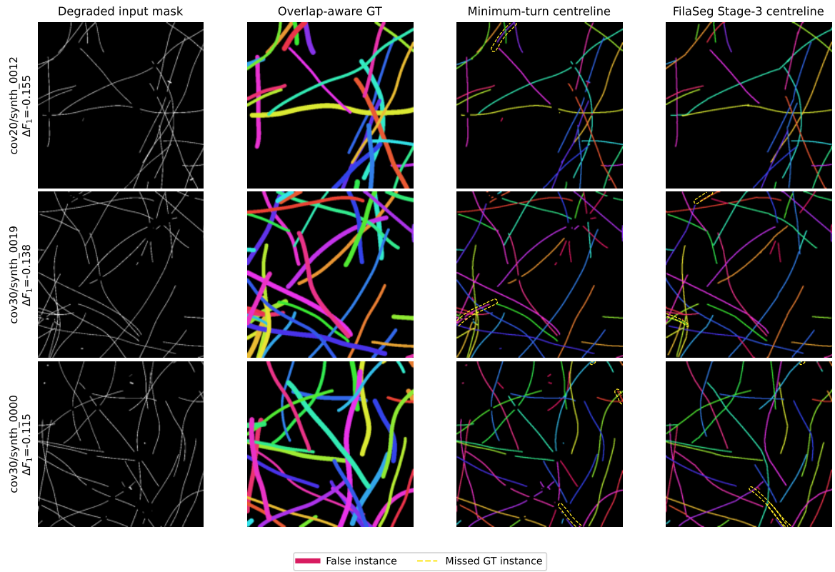
Figure 6. The three predefined synthetic scenes with the largest paired advantages for the minimum-turn tracer. These counterexamples show conditions under which local minimum-turn continuation grouped the visible filament fragments more accurately than FilaSeg. Columns are as in Figure 5. Predicted and reference centrelines are drawn with a 3-pixel display-only dilation for print legibility; the underlying one-pixel skeletons used for matching and scoring are unchanged.
