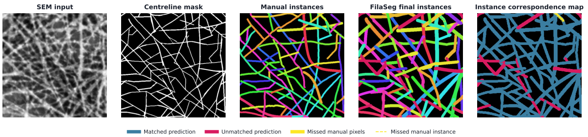
Figure 9. Real SEM development crop. Corresponding manual reference and predicted instances use the same colours after maximum-total-IoU one-to-one assignment. Magenta indicates unmatched predictions, while a dashed yellow outline indicates the missed manual reference instance. The final panel summarizes instance correspondence without treating apparent-width disagreement as a centreline-grouping error.
