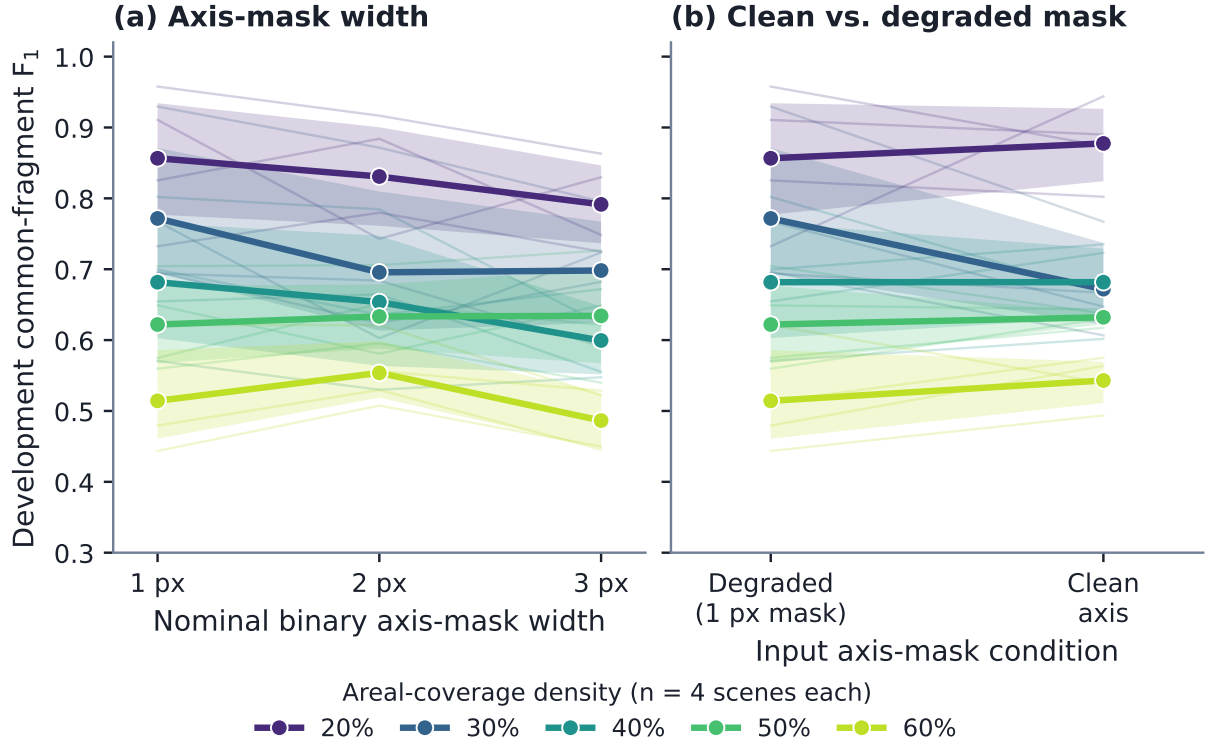
Figure 7. Development-only sensitivity of the common-fragment F_1 to the input mask representation, resolved by prescribed areal coverage. (a) nominal binary filament-axis width of exactly one, two and three pixels. (b) clean versus degraded one-pixel axis masks. Each of the five curves is the mean over the four development scenes belonging to one coverage level ( n = 4 per level, 20 scenes in total). The same scenes recur at every horizontal position, so the shaded 95% confidence intervals come from a percentile bootstrap that resamples scenes within a coverage level and reuses the resampled scene set across positions, preserving the within-scene pairing (10 000 replicates, fixed seed). Individual scenes are drawn lightly behind the means. The two panels share the vertical scale and the legend, but their horizontal axes are different conditions and are deliberately not pooled. With four scenes per level these are sensitivity diagnostics, not precise estimates.
