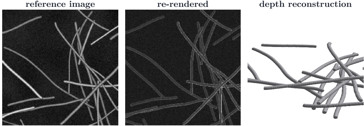
Figure 11. The depth stage on one synthetic scene, reconstructed from the binary axis mask. The image the scene was rendered from, that scene re-rendered from the reconstruction through a forward SEM model, and the film the reconstruction implies. The re-rendered panel is a consistency check on depths and radii, not a scored quantity: the difference Table 6 reports between input conditions is a difference in which crossings were found , which a rendered image cannot show. The table carries that measurement.
