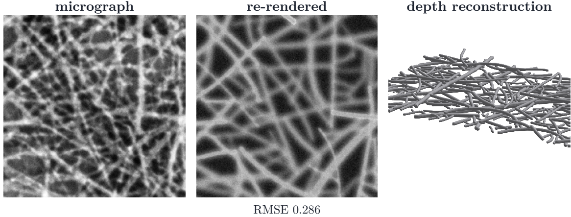
Figure 12. The same comparison on a real CNT SEM field, reconstructed from the axis of annotator A’s annotation. Nothing here is scored. No depth ground truth exists for real SEM – the annotation records which pixels belong to which strand, not which strand lies on top, so this shows the stage runs end to end on real data and re-renders to something recognisable, not that the depths are right. The forward model’s appearance parameters are fitted to this micrograph, so the residual quoted beneath the panel is in-sample and is a sanity check rather than a measure of reconstruction quality.
