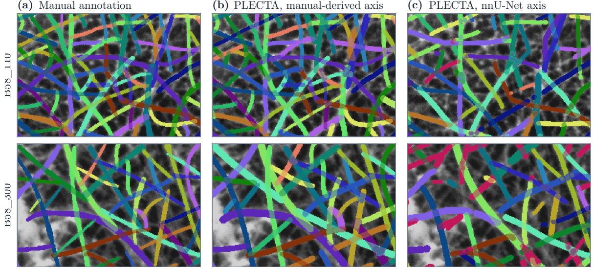
Figure 10. Reconstructed bundles on two of the annotated SEM fields, one field per row. (a) annotator A’s annotation; (b) PLECTA from the manual-derived axis; (c) PLECTA from the nnU-Net axis of Figure 9b, the same method and the same parameters, differing only in the mask. All three are drawn at width so that they are the same kind of object: the annotation as the annotator painted it, and the two reconstructions through the optional image layer of Section 2.5.1, which measures a width per strand across the centreline and renders a ribbon. That layer runs after the grouping is fixed and cannot move a pixel from one strand to another, so no score in this paper depends on it. Strand colours correspond across the panels of a row: a predicted strand takes the colour of the annotated strand it was matched to, one matched to none is crimson, and adjacent strands are given different colours, which carry identity within the row and nothing else. Each crop is the window whose local pairwise F_1 is jointly closest to that field’s whole-field value on both axes, so it is typical of the field rather than selected from it.
