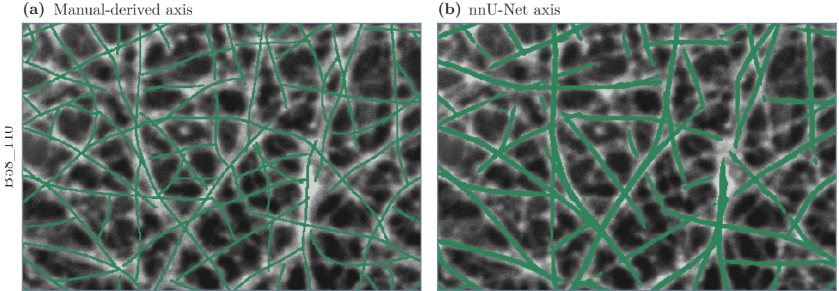
Figure 9. The two input axes of field B58_110, drawn over the micrograph they were read from: (a) the skeleton of annotator A’s annotation and (b) the output of Pipeline A. These are the binary masks themselves, before any reconstruction, so there is nothing to tell apart within a panel and one colour is sufficient; the comparison the figure makes is between them. Everything separating the two conditions of Table 5 is visible here: the same strands, read a second time by a network rather than by a person, arrive thicker, broken into more pieces, and displaced by a pixel or two almost everywhere. The axis is dilated by one pixel for legibility at this size, which changes no geometry. B58_300 behaves the same way, as its mask-quality triple in the text records.
