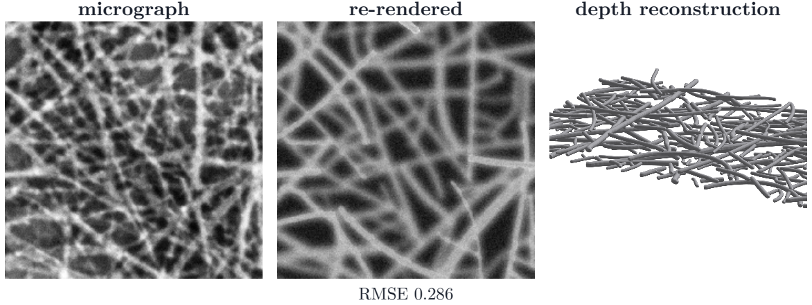
Figure 9. The same comparison on a real CNT SEM field, reconstructed from the axis of annotator A’s annotation. Nothing here is scored. No depth ground truth exists for real SEM – the annotation records which pixels belong to which strand, not which strand lies on top, so this shows the stage runs end to end on real data and re-renders to something recognisable, not that the depths are right. The forward model’s appearance parameters are fitted to this micrograph, so the residual quoted beneath the panel is in-sample and is a sanity check rather than a measure of reconstruction quality.
