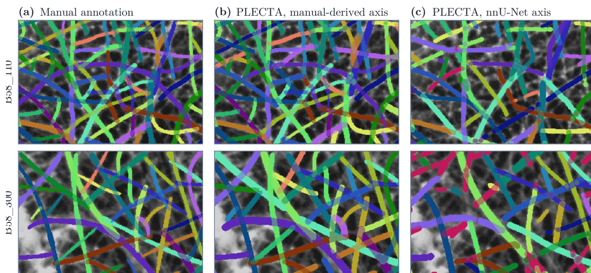
Figure 7. Reconstructed bundles on two of the annotated SEM fields, one field per row. (a) annotator A’s annotation; (b) PLECTA from the manual-derived axis; (c) PLECTA from the nnU-Net axis of Figure 6b, the same method and the same parameters, differing only in the mask. All three are drawn at width so that they are the same kind of object: the annotation as the annotator painted it, and the two reconstructions through the optional image layer of Section 2.5, which measures a width per strand across the centreline and renders a ribbon. That layer runs after the grouping is fixed and cannot move a pixel from one strand to another, so no score in this paper depends on it. Strand colours correspond across the panels of a row: a predicted strand takes the colour of the annotated strand it was matched to, one matched to none is crimson, and adjacent strands are given different colours, which carry identity within the row and nothing else. Each crop is the window whose local pairwise F_1 is jointly closest to that field’s whole-field value on both axes, so it is typical of the field rather than selected from it.
