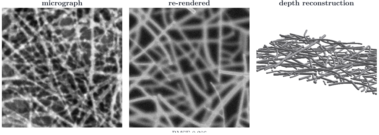
Figure 10. The same comparison on a real CNT SEM field, reconstructed from the axis of annotator A’s annotation. Nothing here is scored: real SEM has no depth ground truth, since the annotation records which pixels belong to which strand, not which lies on top. It shows that the stage runs end to end and re-renders to something recognisable, not that the depths are right. The forward model’s appearance parameters are fitted to this micrograph, so the residual beneath the panel is in-sample.
