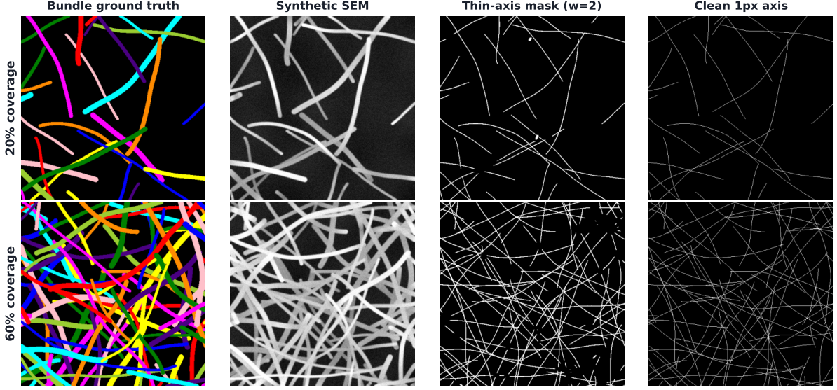
Figure 2. Examples of the procedural synthetic data. Each row shows the overlap-aware thick-instance reference, an SEM-like grayscale image, the a degraded thin-axis mask of the kind supplied to FilaSeg, and the undegraded one-pixel axis representation. The degraded example is shown at a nominal two-pixel axis width to make the degradation visible; the primary evaluation uses the nominal one-pixel variant. The geometric instance identity is retained across all representations.
