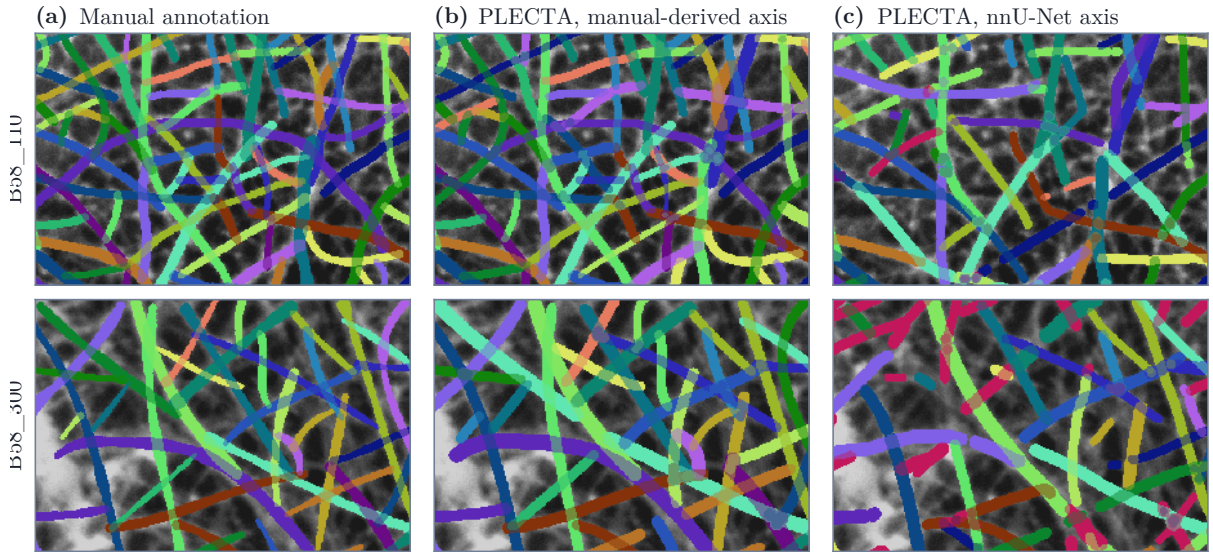
Figure 7. Reconstructed bundles on two of the annotated SEM fields, one field per row. (a) reader A’s annotation; (b) PLECTA from the manual-derived axis; (c) PLECTA from the nnU-Net axis of Figure 6b, the same method and the same parameters, differing only in the mask. All three are drawn at width so that they are the same kind of object: the annotation as the annotator painted it, and the two reconstructions through the optional image layer of Section 2.5, which measures a width per strand across the centreline and renders a ribbon. That layer runs after the grouping is fixed and cannot move a pixel from one strand to another, so no score in this paper depends on it. Strand colours correspond across the panels of a row: a predicted strand takes the colour of the annotated strand it was matched to, one matched to none is crimson, and adjacent strands are given different colours, which carry identity within the row and nothing else. Each crop is the window whose local pairwise F_1 is jointly closest to that field’s whole-field value on both axes, so it is typical of the field rather than selected from it.
