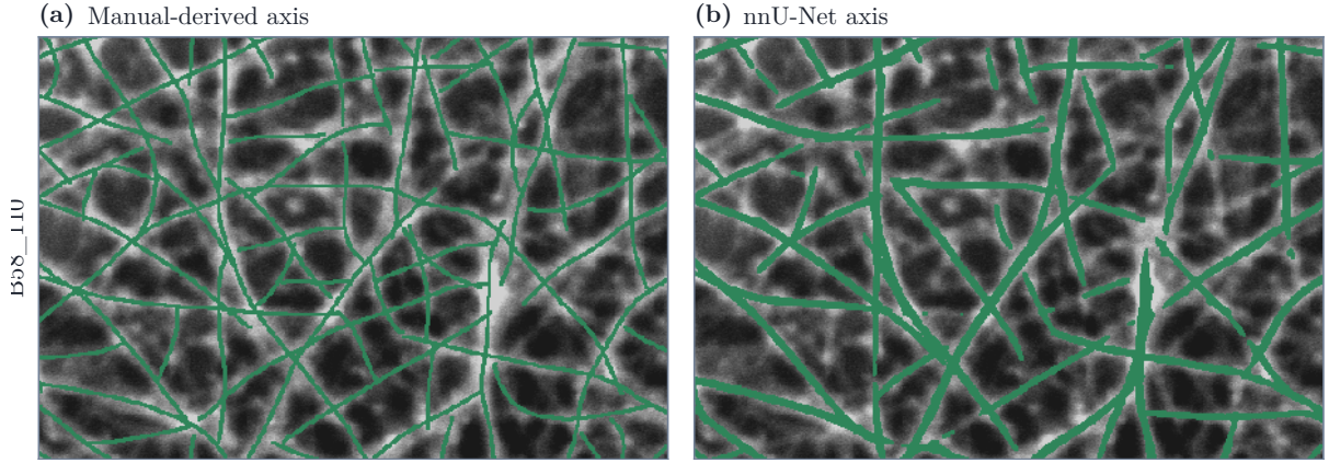
Figure 6. The two input axes of field B58_110, drawn over the micrograph they were read from: (a) the skeleton of reader A’s annotation and (b) the output of Pipeline A. These are the binary masks themselves, before any reconstruction, so there is nothing to tell apart within a panel and one colour is sufficient; the comparison the figure makes is between them. Everything separating the two conditions of Table 5 is visible here: the same strands, read a second time by a network rather than by a person, arrive thicker, broken into more pieces, and displaced by a pixel or two almost everywhere. The axis is dilated by one pixel for legibility at this size, which changes no geometry. B58_300 behaves the same way, as its mask-quality triple in the text records.
