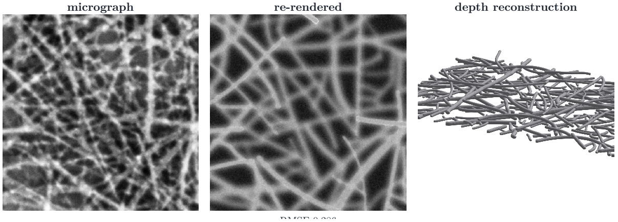
Figure 12. The same comparison on a real CNT SEM field, reconstructed from the axis of annotator A’s annotation. Nothing here is scored. No depth ground truth exists for real SEM – the annotation records which pixels belong to which strand, not which strand lies on top, so this shows the stage runs end to end on real data and re-renders to something recognisable, not that the depths are right. The forward model’s appearance parameters are fitted to this micrograph, so the residual quoted beneath the panel is in-sample and is a sanity check rather than a measure of reconstruction quality.
