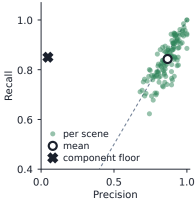
(c) Precision vs. recall
