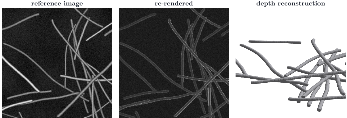
Figure 8. The depth stage on one synthetic scene, reconstructed from the binary axis mask. The image the scene was rendered from, that scene re-rendered from the reconstruction through a forward SEM model, and the film the reconstruction implies. The re-rendered panel is a consistency check on depths and radii, not a scored quantity: the difference Table 2 reports between input conditions is a difference in which crossings were found , which a rendered image cannot show. The table carries that measurement.
