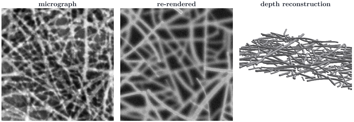
Figure 12. The same comparison on a real CNT SEM field, reconstructed from the axis of annotator A’s annotation. Nothing here is scored. No depth ground truth exists for real SEM – the annotation records which pixels belong to which strand, not which strand lies on top, so this shows the stage runs end to end on real data and re-renders to something recognisable, not that the depths are right. The forward model’s appearance parameters are fitted to this micrograph, so the residual quoted beneath the panel is in-sample and is a sanity check rather than a measure of reconstruction quality.
