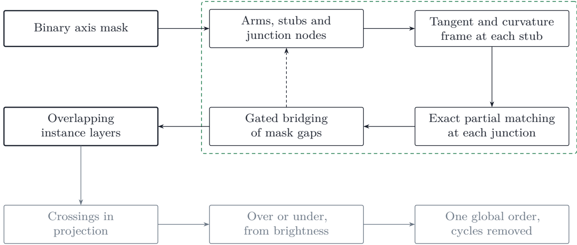
Figure 1. Scope of PLECTA. The dashed grouping stage maps a binary axis mask to overlapping instances; the loop denotes eight rounds of frame refitting and matching. The grey branch uses a paired greyscale image to infer depth order without changing strand identity.
