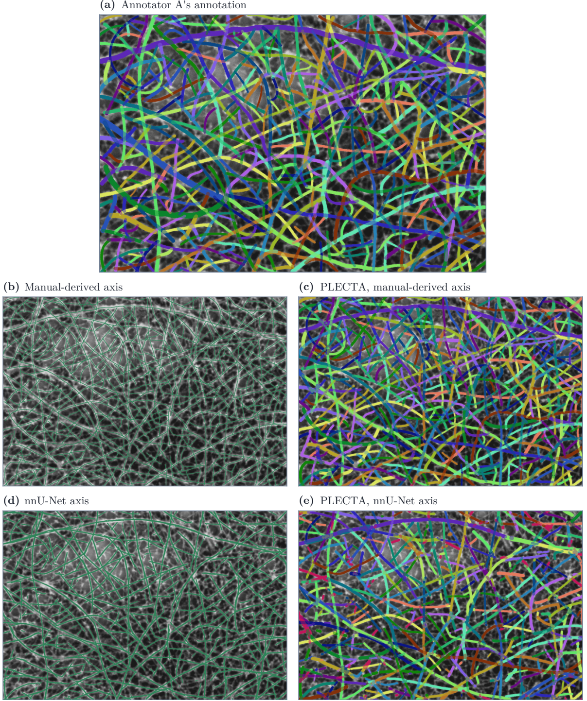
Figure 11. One annotated SEM field, B58_110, whole frame, with a row per mask source. (a) annotator A's annotation; (b) the skeleton of that annotation, which is the manual-derived axis, and (c) PLECTA from it; (d) the output of the upstream segmenter, and (e) PLECTA from that, at the same parameters. Panels (b) and (d) are the input masks themselves, before any reconstruction, and everything separating the two conditions of Table 3 is between them: the same strands, read by a network rather than by a person, arrive thicker, broken into more pieces, and displaced by a pixel or two almost everywhere. They are drawn in one colour and dilated by one pixel for legibility, which changes no geometry. The other three are drawn at width, the reconstructions through the width layer of Section 2.5.1, which runs after the grouping is fixed and moves no pixel between strands; a predicted strand takes the colour of the annotated strand it matched, and crimson matched none. B58_110 is one of the 2 fields the segmenter was not trained on, and the rest are in Table 3 rather than in a second picture.
