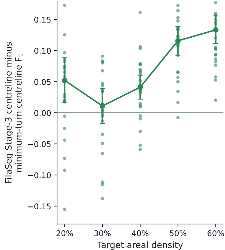
Paired scene differences
