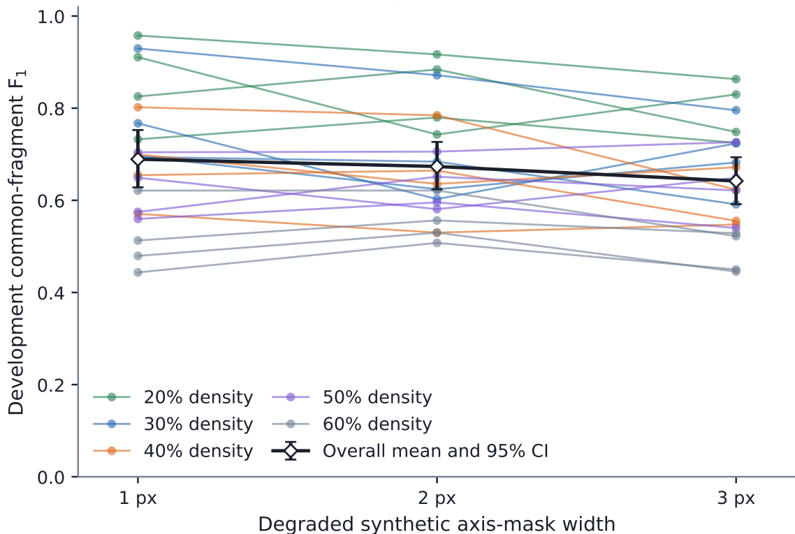
Input-mask width sensitivity (development scenes; n = 20)
