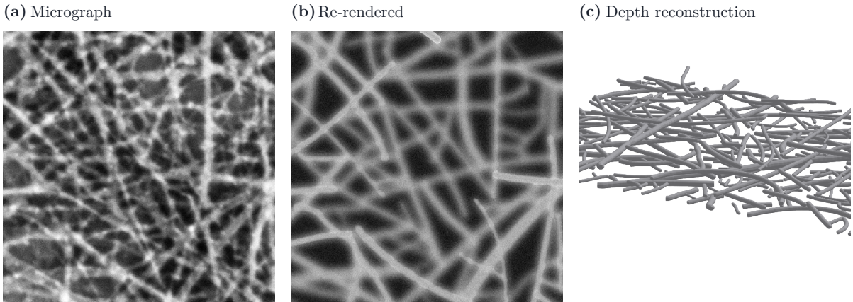
Figure 9. The same comparison on a real CNT SEM field, reconstructed from the axis of annotator A’s annotation; the crop is 512 px across, about 0.55\text{ }\mu\text{m} of field B58_100. The depth order is not evaluated quantitatively here: real SEM provides no depth ground truth, since the annotation records which pixels belong to which strand, not which lies on top. The panels demonstrate the stage running end to end on real imaging; the forward model’s appearance parameters are fitted to this micrograph.
