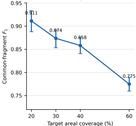
(a) Held-out performance
