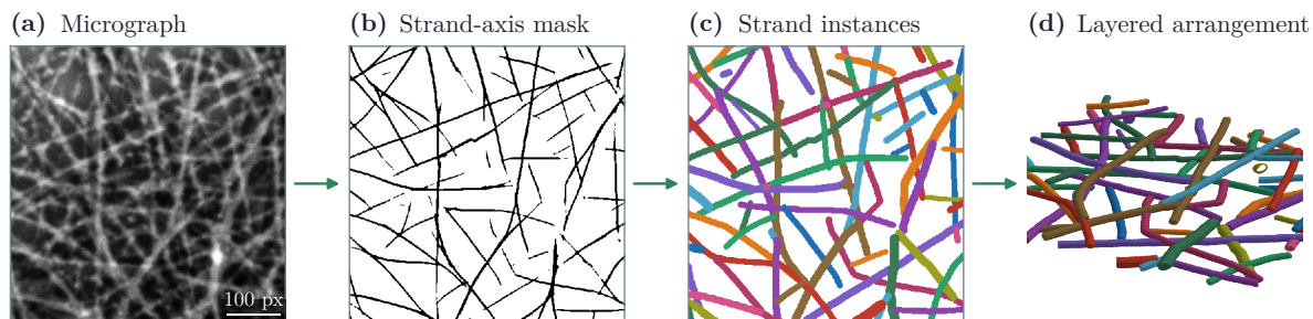
Figure 1. From micrograph to individual strands, on one carbon-nanotube SEM field held out of the segmenter’s training data. (a) A fixed central crop. (b) The strand-axis mask from the upstream segmenter. (c) The instances PLECTA reconstructs from that mask alone, each drawn at the width measured for it across its own centreline. (d) The layered arrangement estimated for the same instances, at the same widths and without vertical exaggeration. Colour carries instance identity in both (c) and (d) and nothing else.
