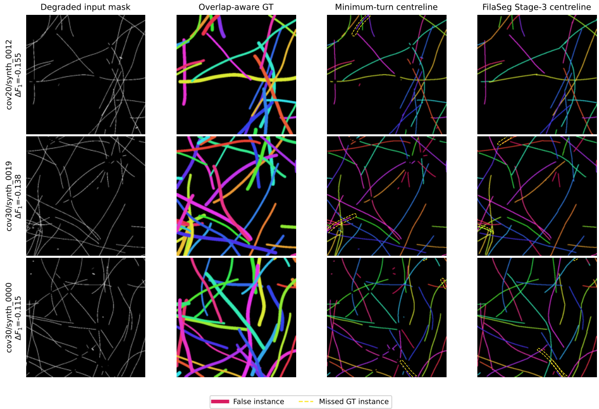
Figure 6. The three predefined synthetic scenes with the largest paired advantages for the minimum-turn tracer, selected from the stored numerical differences and not by visual inspection. Columns are as in Figure 5. Predicted and reference centrelines are drawn with a 3-pixel display-only dilation for print legibility; the underlying one-pixel skeletons used for matching and scoring are unchanged.
