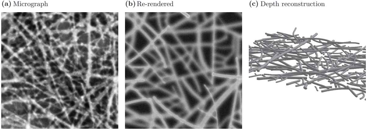
Figure 10. The same comparison on a real CNT SEM field, reconstructed from the reference axis mask. The crop is 512 px across, about 0.55\text{ }\mu\text{m} of field B58_100. Real SEM provides no depth ground truth, so the depth order is shown qualitatively; the forward-model appearance parameters are fitted to this micrograph.
