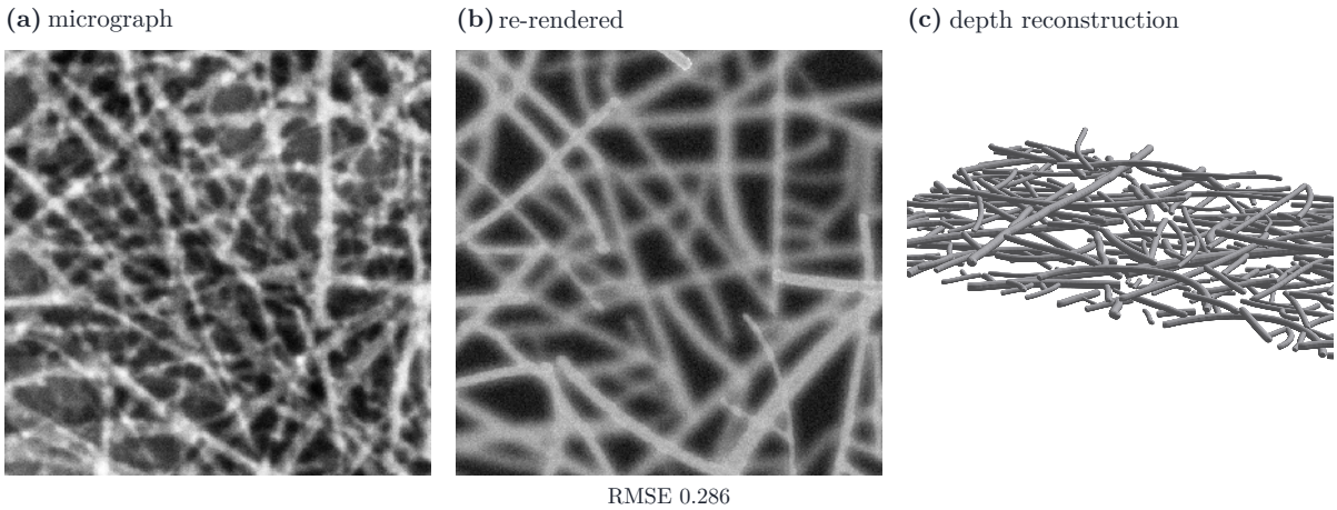
Figure 9. The same comparison on a real CNT SEM field, reconstructed from the axis of annotator A’s annotation. Nothing here is scored: real SEM has no depth ground truth, since the annotation records which pixels belong to which strand, not which lies on top. It shows that the stage runs end to end and re-renders to something recognisable. The forward model’s appearance parameters are fitted to this micrograph, so the residual beneath the panel is in-sample.
