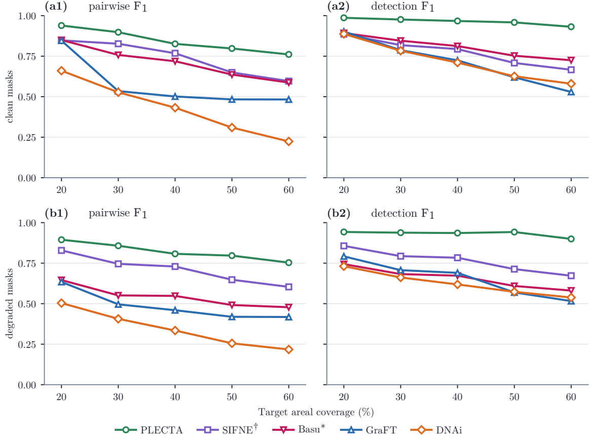
Figure 4. Five methods on identical masks, by coverage stratum: (a) the undegraded axis, (b) the degraded one; columns are pairwise F_1 , which counts pairs of fragments, and detection F_1 at IoU 0.1 with a 2 px tolerance, which counts objects (Section 2.7). The two disagree where a method fragments, since only the first is quadratic in fragmentation. Crossing Fidelity is in Table 3. Means of ten scenes, no interval claimed. ^\dagger released source, our development-selected parameters; ^* our reimplement, never released.
