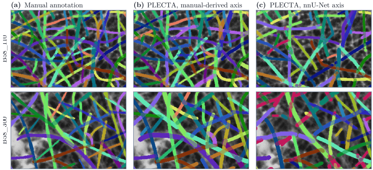
Figure 7. Reconstructed bundles on two of the annotated SEM fields, one field per row. (a) the manual annotation; (b) PLECTA from the manual-derived axis; (c) PLECTA from the nnU-Net axis of Figure 6b, the same method and the same parameters, differing only in the mask. All three are drawn at width so that they are the same kind of object: the annotation as the annotator painted it, and the two reconstructions through the optional image layer of Section 2.5, which measures a width per strand across the centreline and renders a ribbon. That layer runs after the grouping is fixed and cannot move a pixel from one strand to another, so no score in this paper depends on it. Strand colours correspond across the panels of a row: a predicted strand takes the colour of the annotated strand it was matched to, one matched to none is crimson, and adjacent strands are given different colours, which carry identity within the row and nothing else. Each crop is the window whose local pairwise F_1 is jointly closest to that field’s whole-field value on both axes, so it is typical of the field rather than selected from it.
