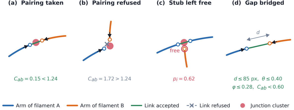
Figure 3. Every decision the linker can make. (a) A junction pairing accepted below the admissibility limit 2p_i . (b) A competing pairing at the same node refused, its cost exceeding 2p_i = 1.24 . (c) A stub left unmatched because paying p_i = 0.62 beats any edge it has. (d) A gap joined between two stubs the junction stage left free, under four gates at once. Idealised drawing; measured values are in Figures 2 and 4.
