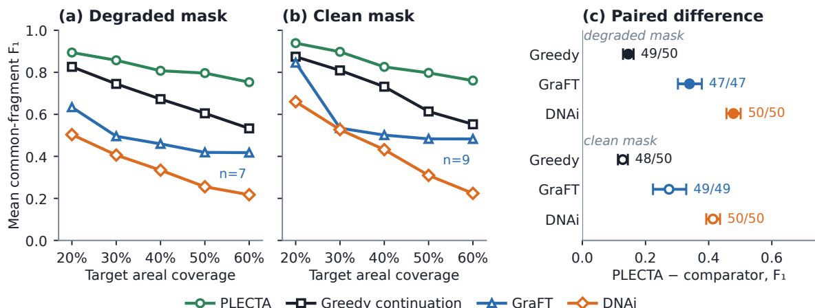
Figure 7. PLECTA against two published methods and a greedy baseline, on the same 50 scenes, the same input masks and one scorer. (a) degraded and (b) clean input mask: mean common-fragment F_1 per coverage stratum, n = 10 scenes per point except where labelled otherwise; plain means, no interval is drawn and none is claimed. GraFT exceeded its per-scene wall-clock budget on 3 of the 50 degraded scenes and 1 of the clean ones; those are excluded from its means and are the hardest of the densest stratum, so the GraFT curve is optimistic. DNAi is shown at the best configuration found for it on development scenes. The greedy baseline uses the gates selected by a sweep over the development scenes. (c) aggregate paired difference with its density-stratified bootstrap 95 % interval (20 000 replicates), filled markers degraded and open markers clean; the fraction beside each interval is the number of scenes on which PLECTA scored higher, out of those both methods completed.
