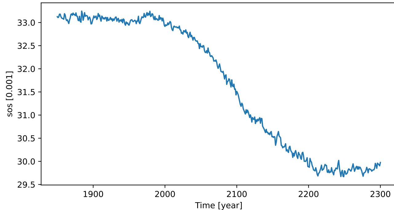
Time series
