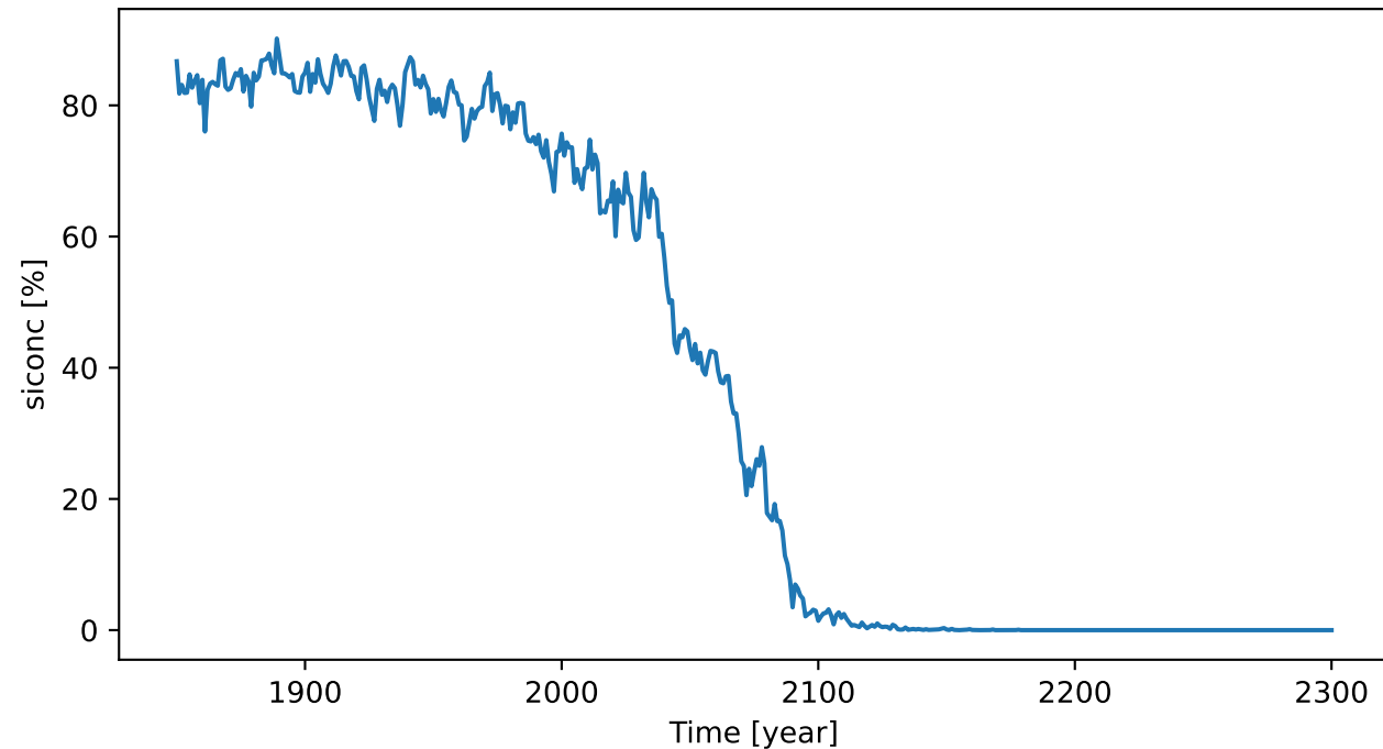
Time series
