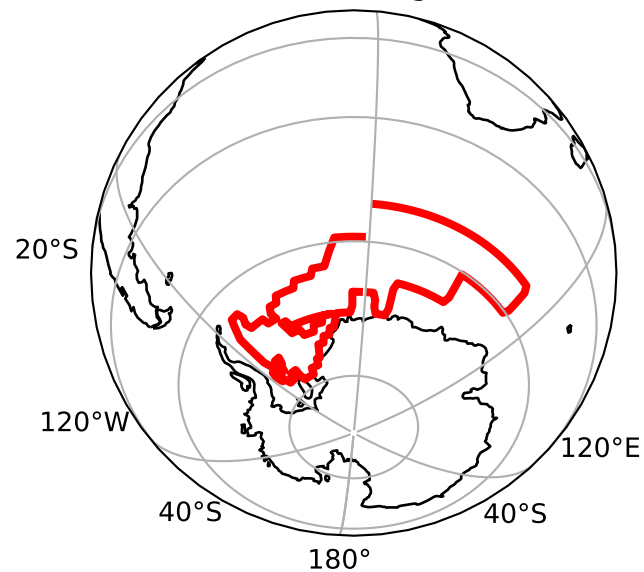
Selected region
