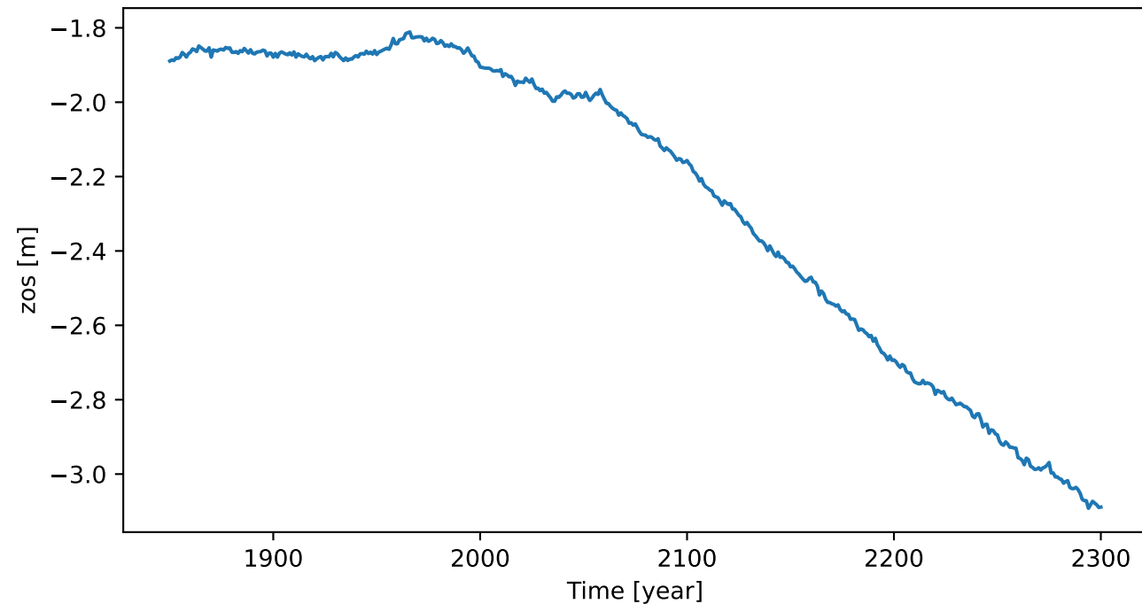
Time series
