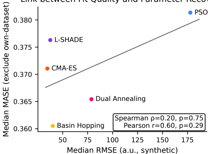
Link between Fit Quality and Parameter Recovery
