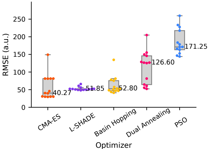
RMSE across 13 runs (AAV)
