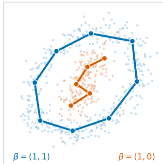
(3) Phase 1: Annealing
