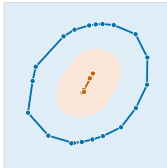
(8) Decision regions
