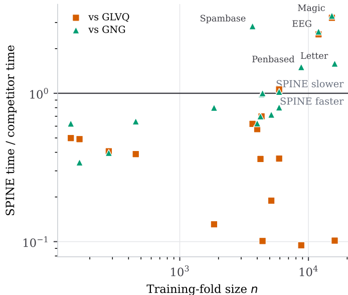
(b) Cost ratio against training-fold size
