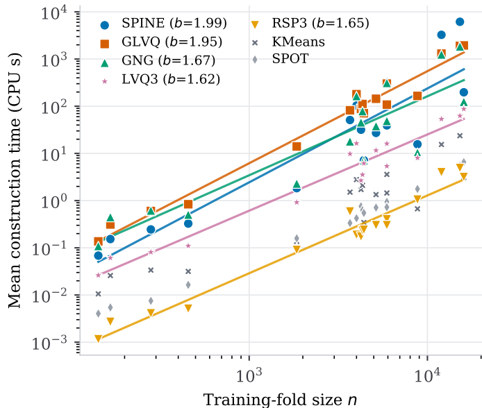
(a) Cost and scaling against training-fold size
