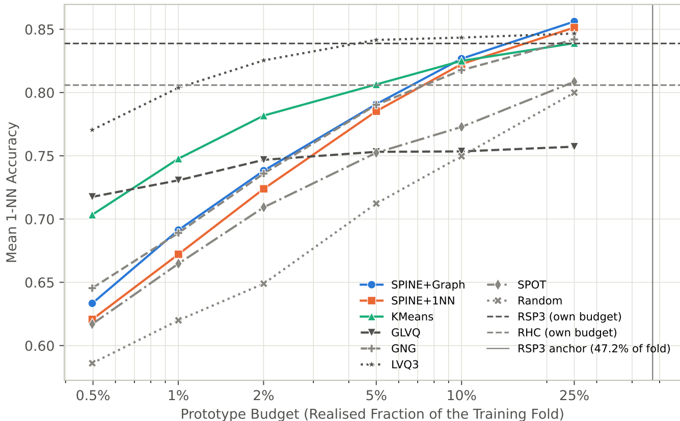
Accuracy against Budget - eeg-eye-state
