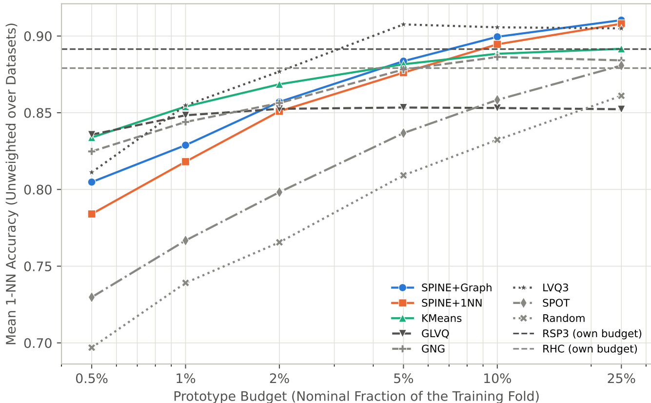
Accuracy against Budget - Average over All Datasets
