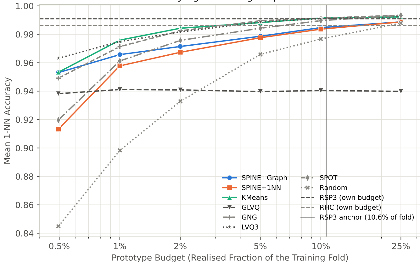
Accuracy against Budget - penbased
