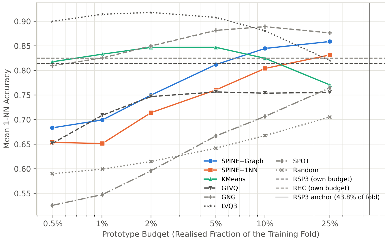
Accuracy against Budget - ring
