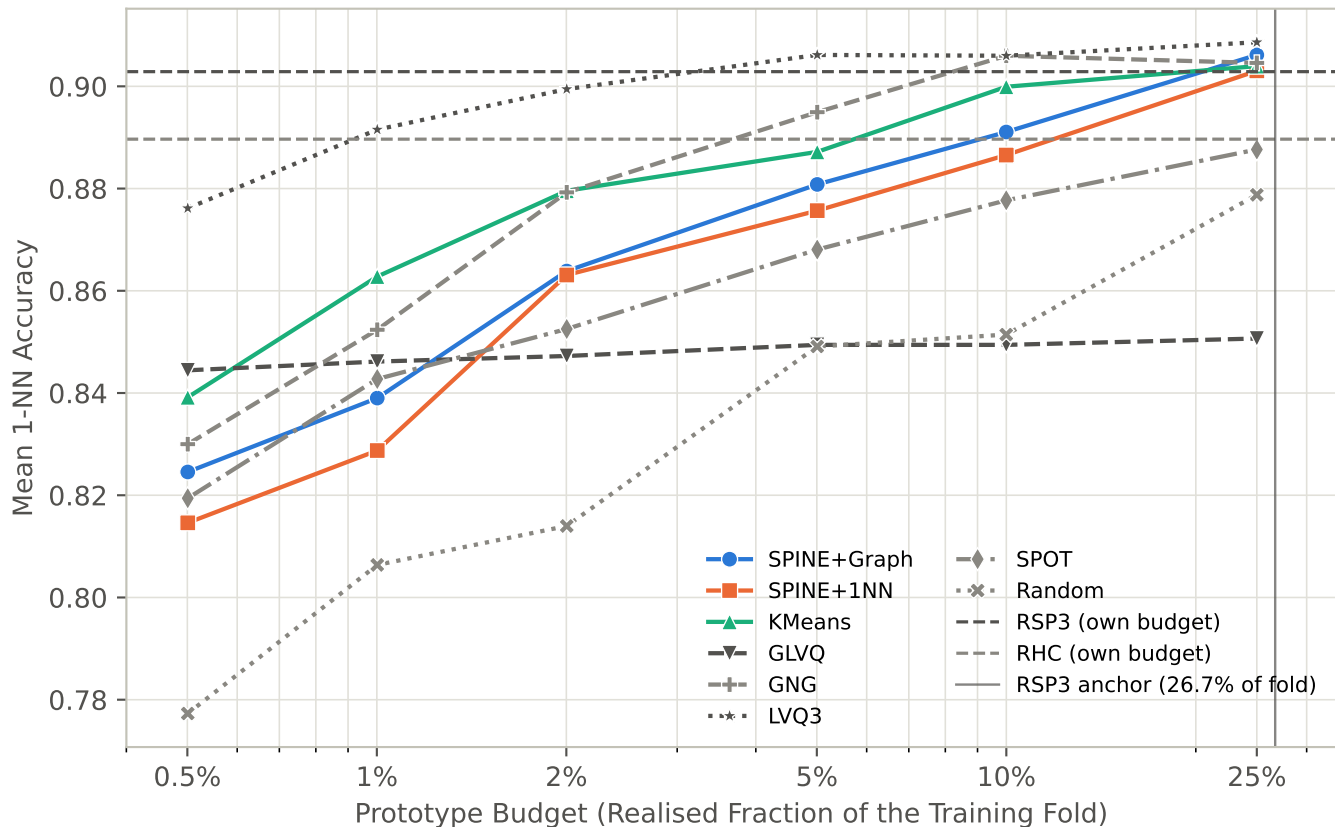
Accuracy against Budget - satimage
