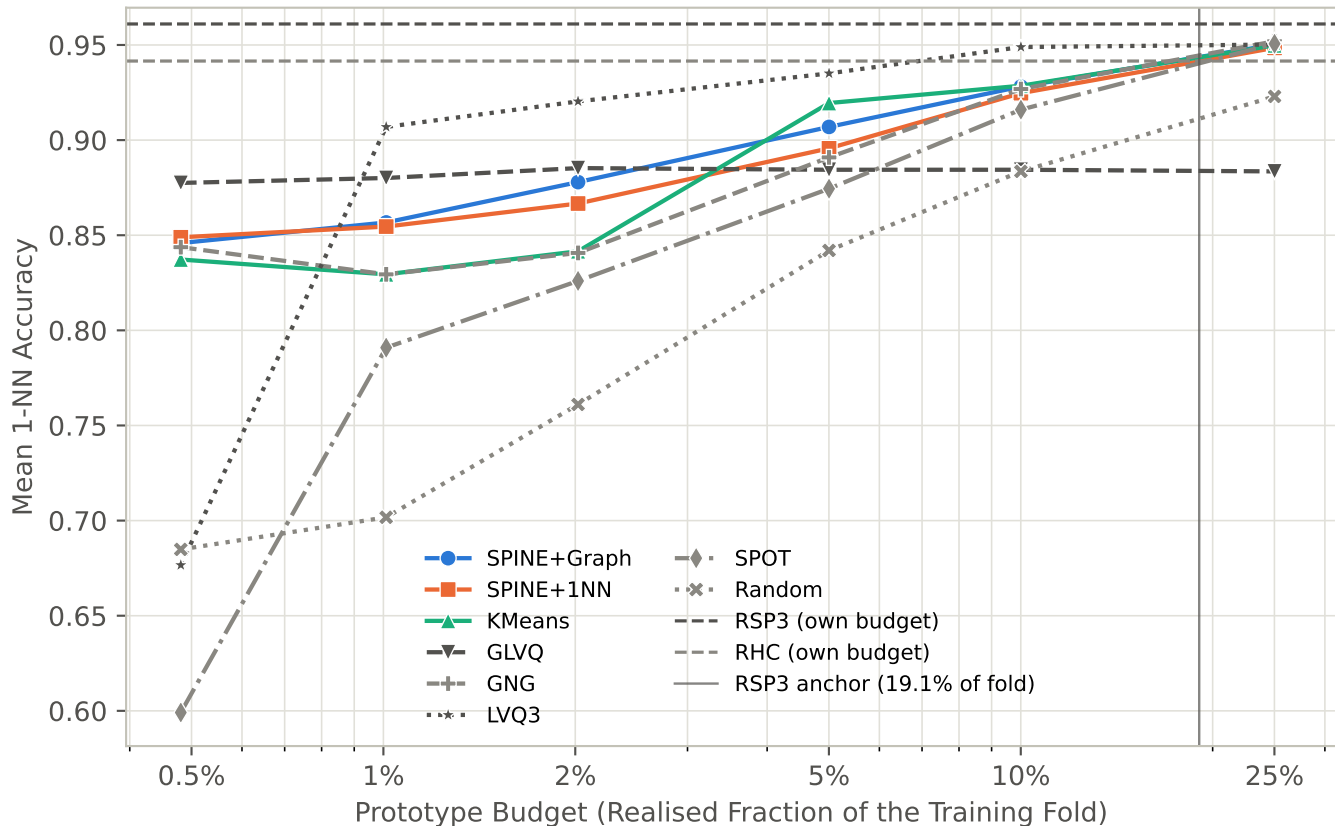
Accuracy against Budget - segment
