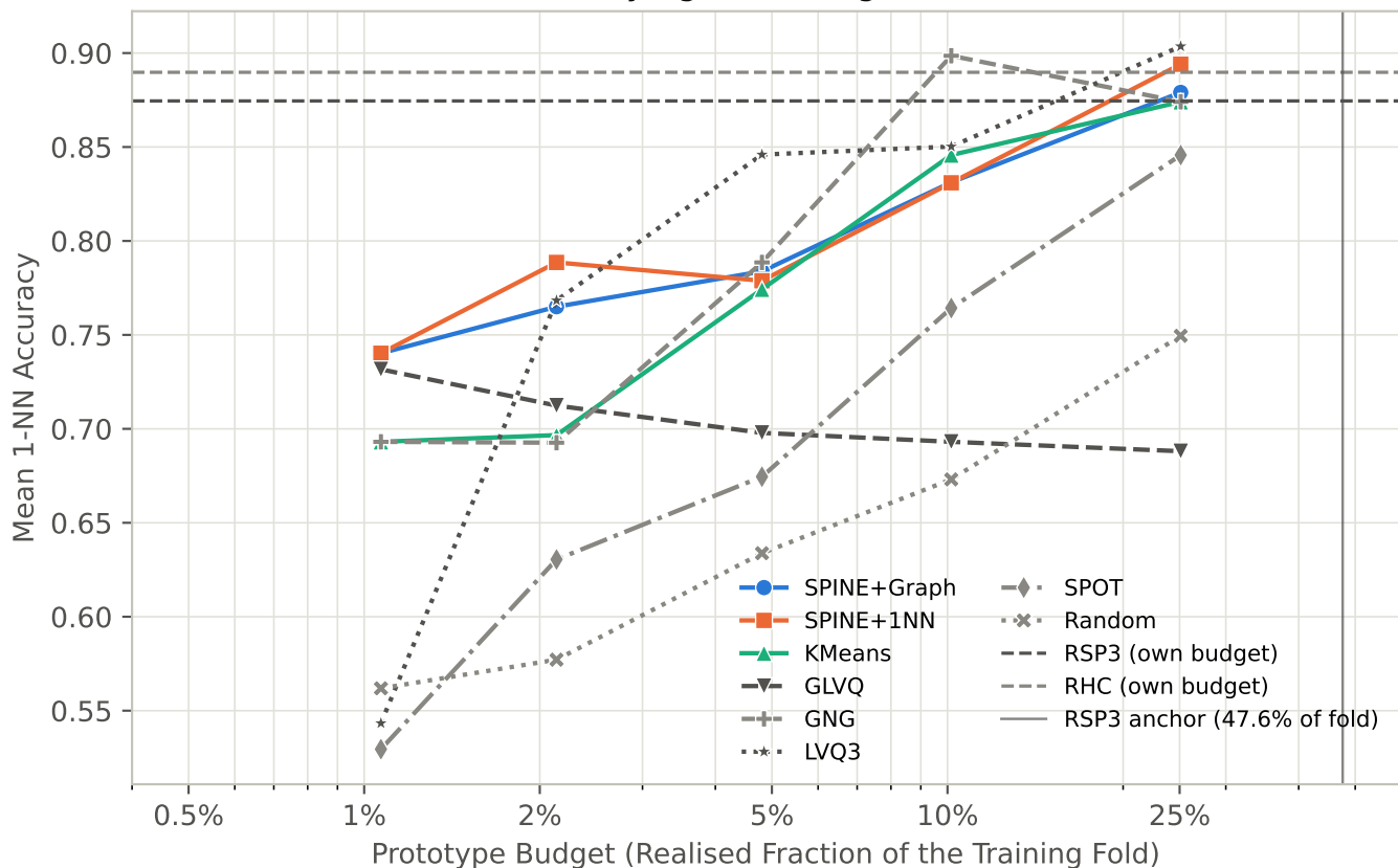
Accuracy against Budget - sonar
