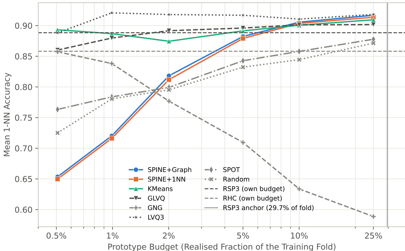
Accuracy against Budget - spambase
