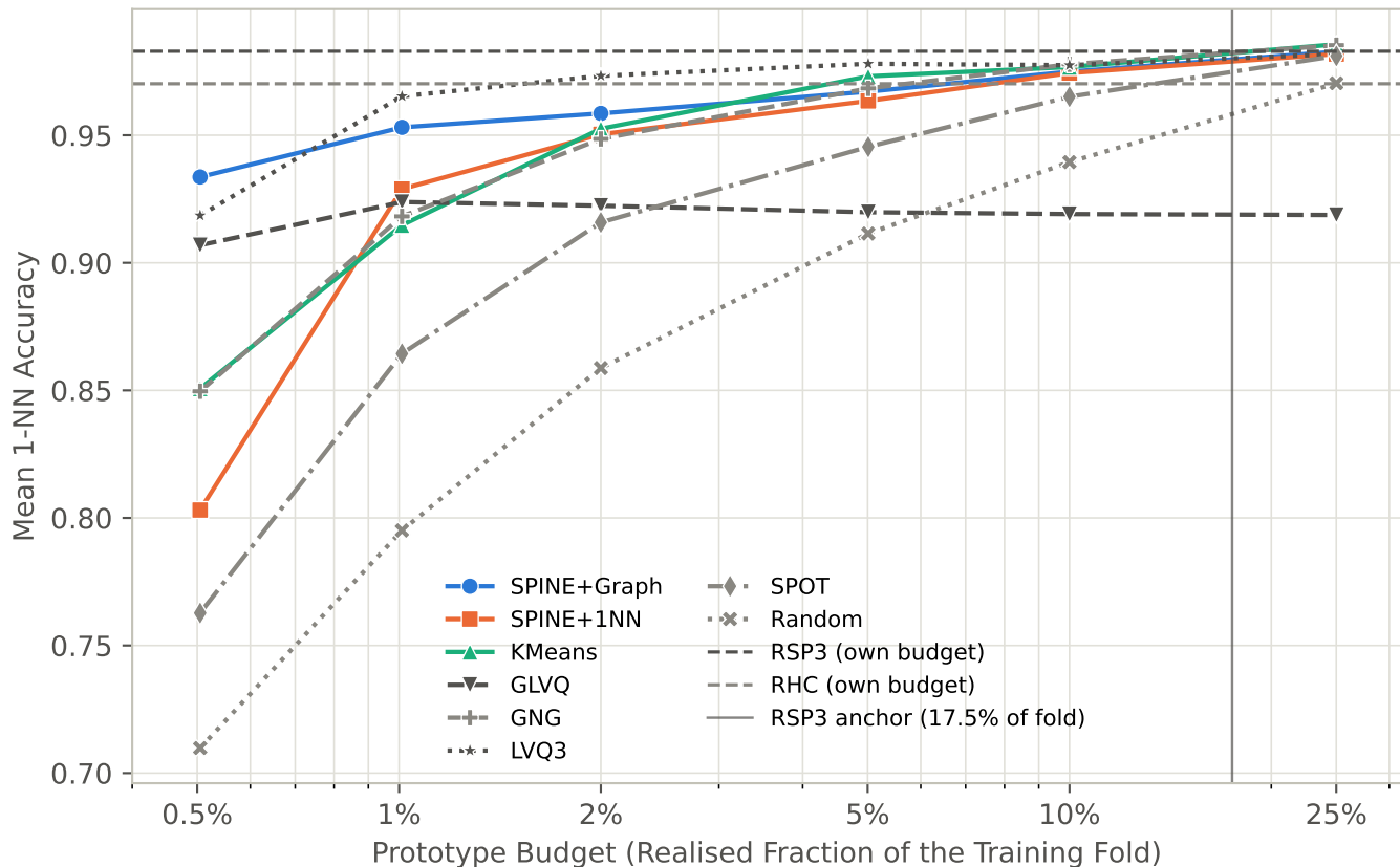
Accuracy against Budget - texture
