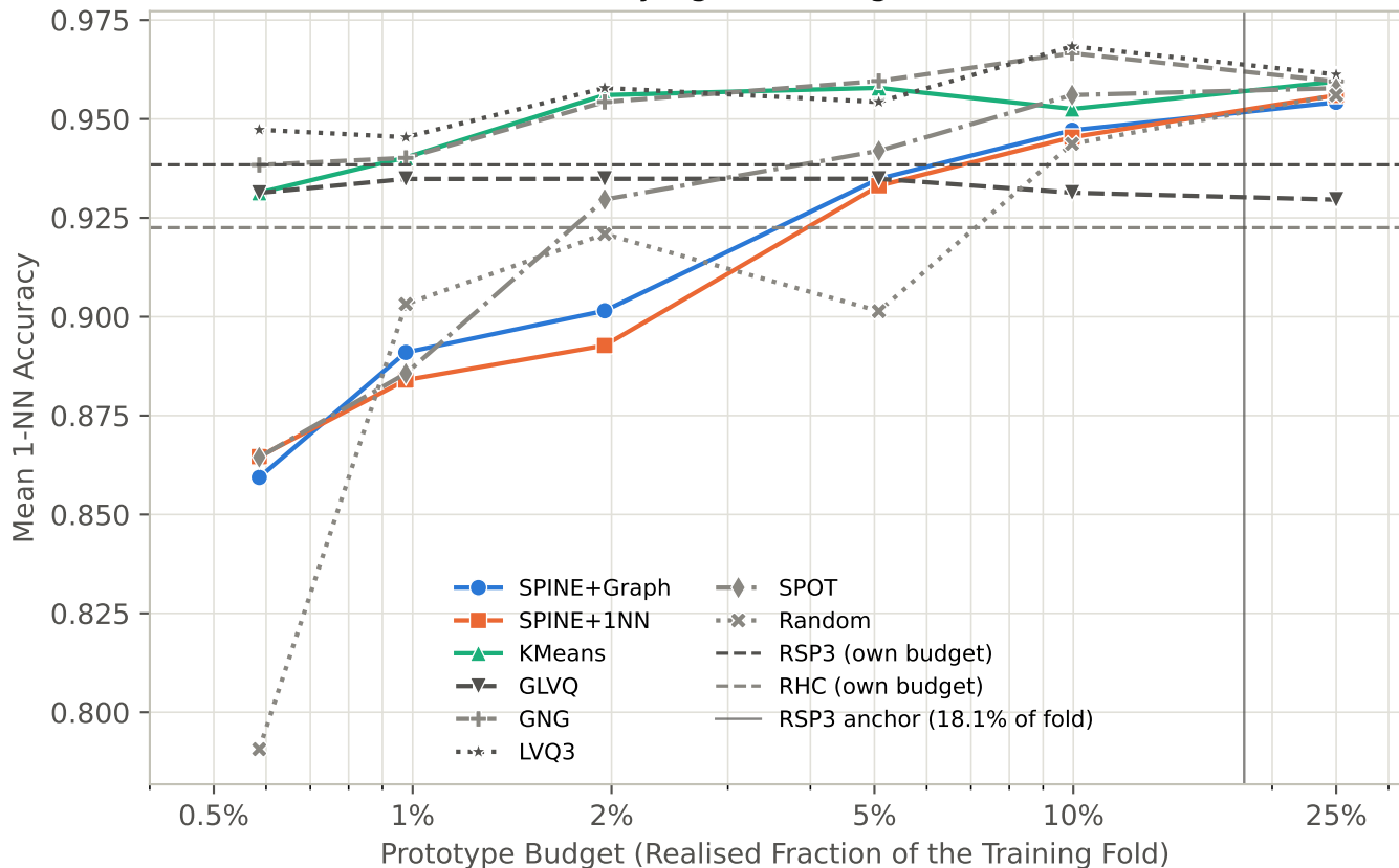
Accuracy against Budget - wdbc
